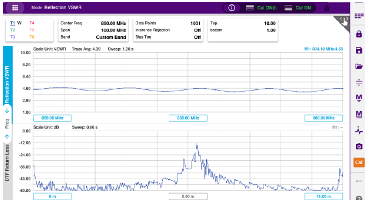
Reflection return loss &amp; smith chart measurement screen (vertical layout)
