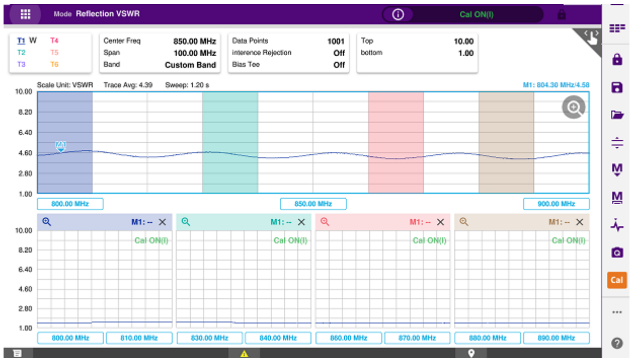
Reflection return loss measurement screen (single layout)
