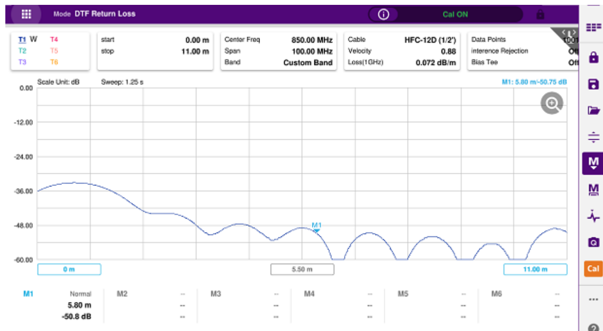
Reflection VSWR & DTF return loss measurement screen (horizontal layout)
