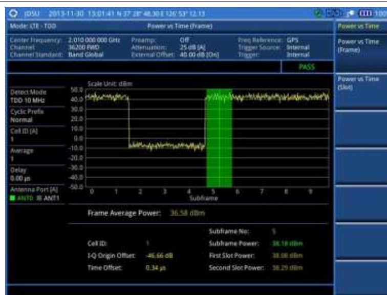
Figure 172 Power vs. time (frame) measurement with LTE – TDD signal analyzer
