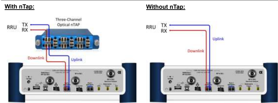
Figure 391 Connection diagram for Layer-2 term testing mode
