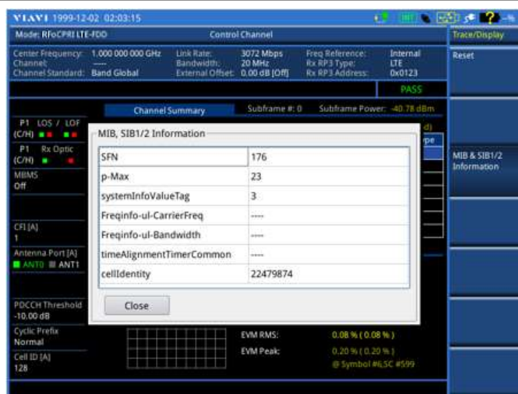
Figure 370 Decoded MIB & SIB1/2 information in RFoCPRI LTE-FDD signal analyzer
