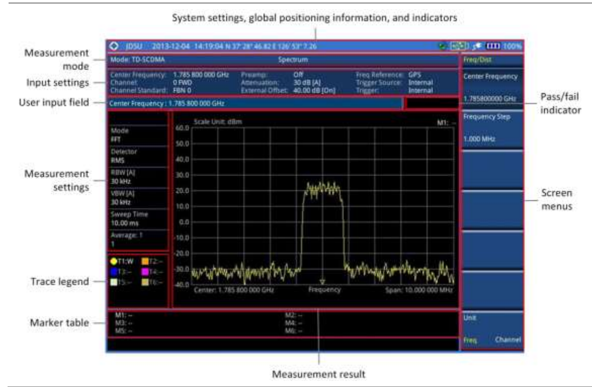
Figure 252 TD-SCDMA signal analyzer measurement screen
