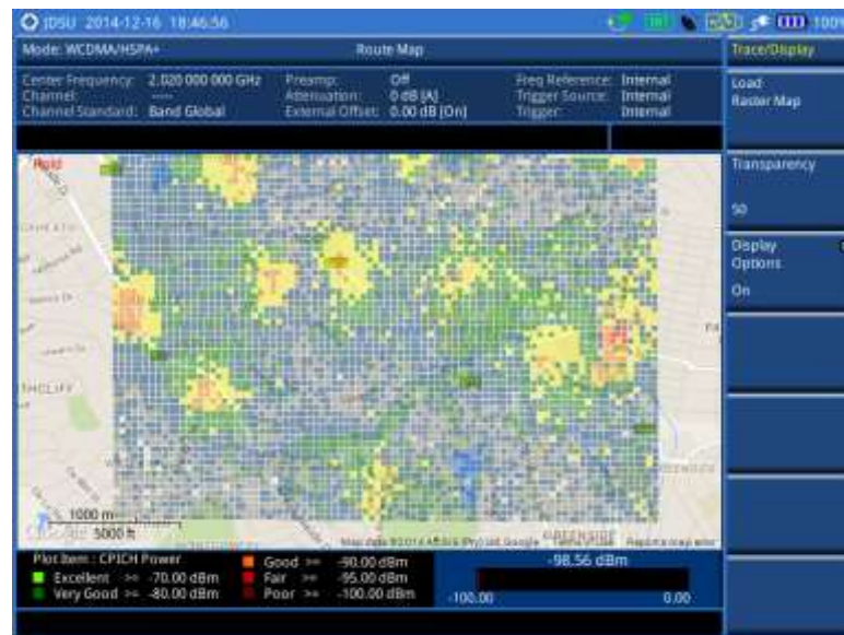
Figure 109 Raster image overlaid on the base map in WCDMA/HSPA+ OTA signal analyzer
