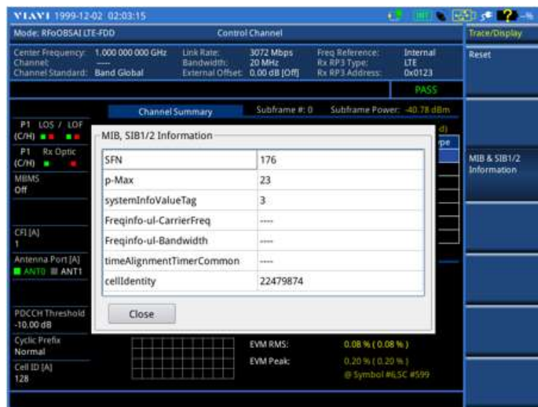
Figure 408 Decoded MIB & SIB1/2 information in RFoBSAI LTE-FDD signal analyzer
