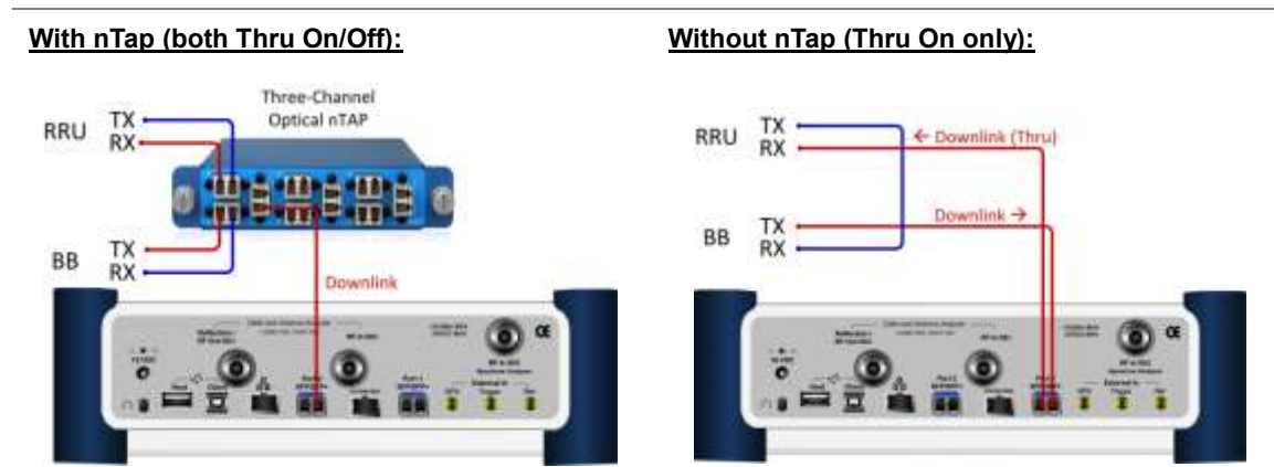
Figure 400 Connection diagram for downlink signal analysis
