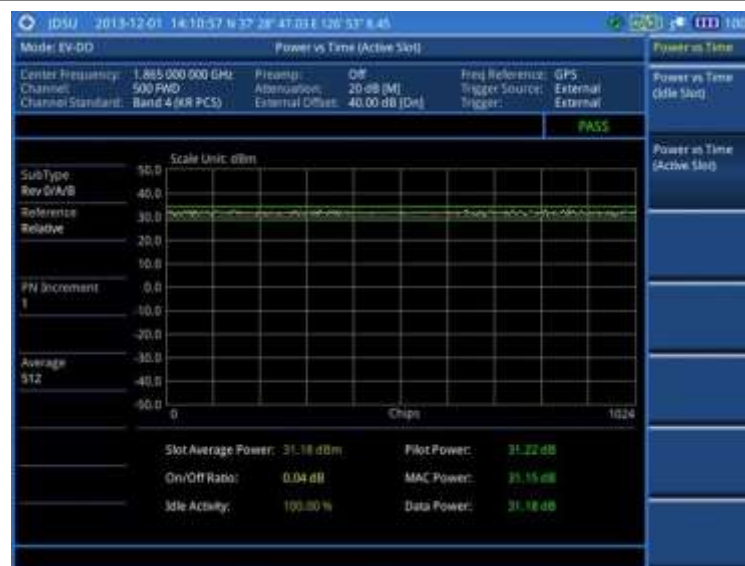
Figure 240 Power vs. time (active slot) measurement with EV-DO signal analyzer
