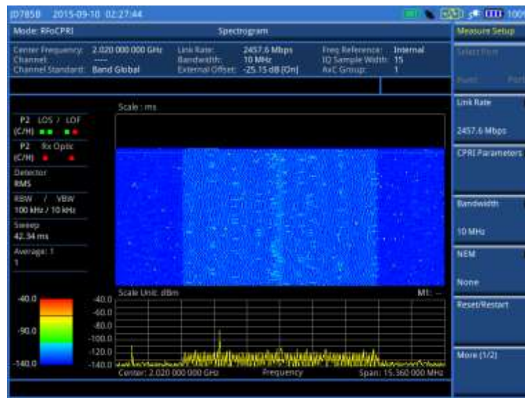
Figure 355 RFoCPRI interference measurement in spectrogram
