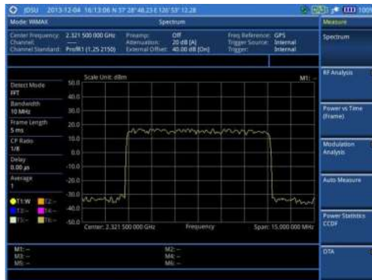
Figure 282 Spectrum measurement screen with Mobile WiMAX signal analyzer
