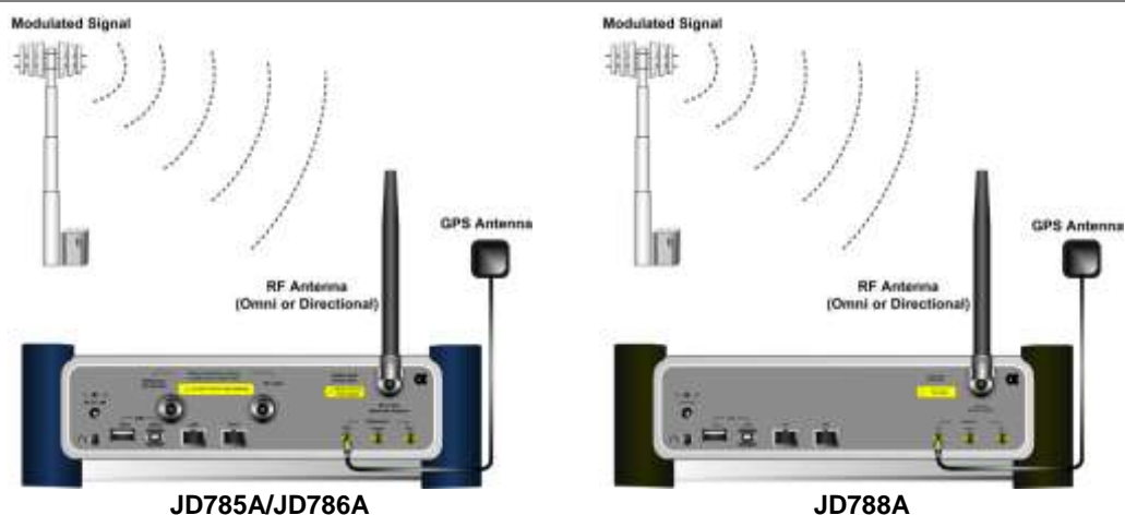
Figure 205 OTA connection
