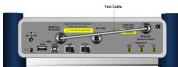
Figure 252 2-port calibration connection in Scalar measurements
