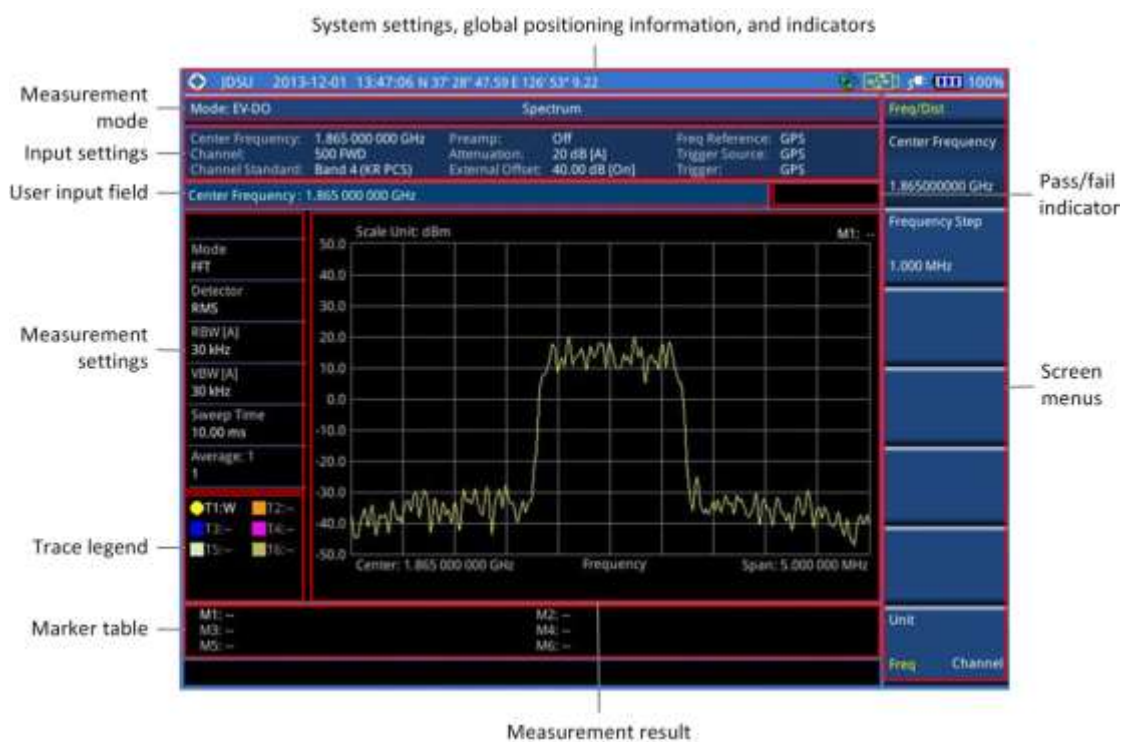
Figure 177 EV-DO signal analyzer measurement screen
