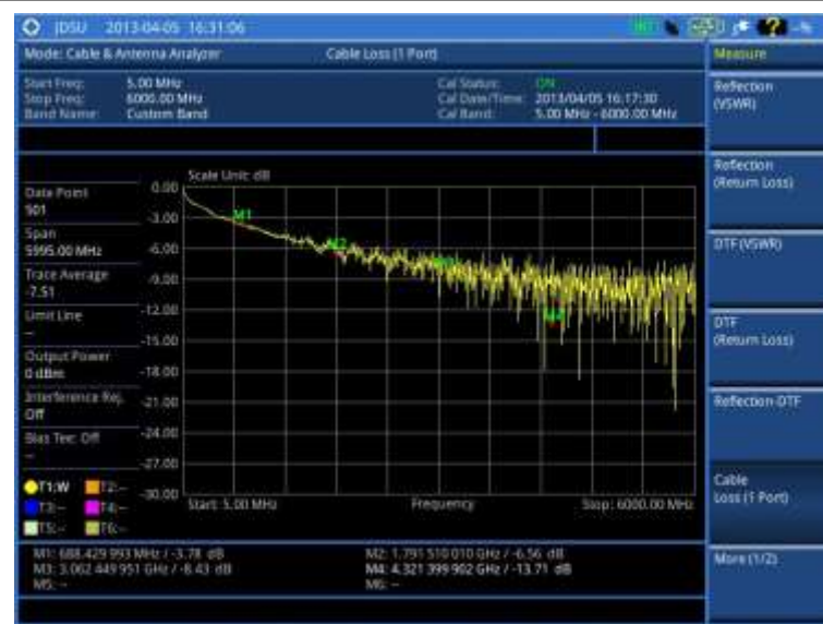
Figure 261 Cable loss (1 port) measurement
