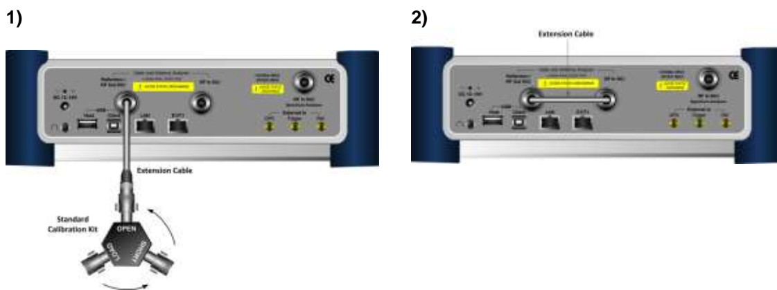
Figure 250 2-port calibration connection with Y-Cal in vector measurements
