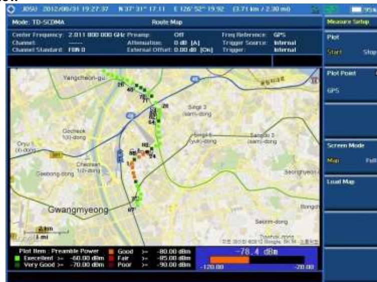
Figure 226 Route map measurement with TD-SCDMA OTA signal analyzer
