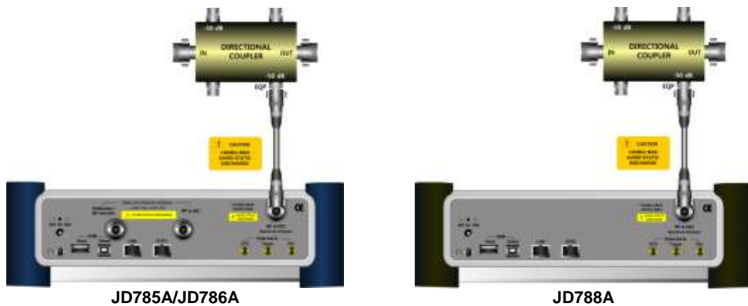
Figure 39 Indirect connection
