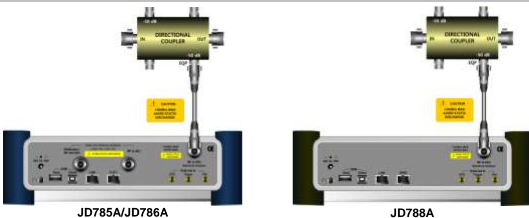
Figure 286 Indirect connection
