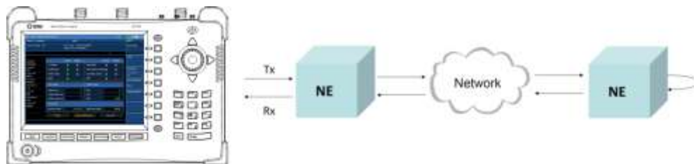
Figure 271 Error injection and measurement connection
