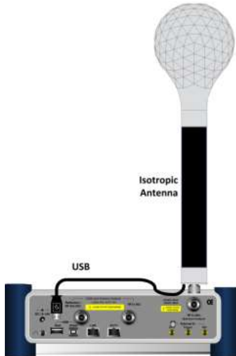
Figure 304 Connection using an isotropic antenna
