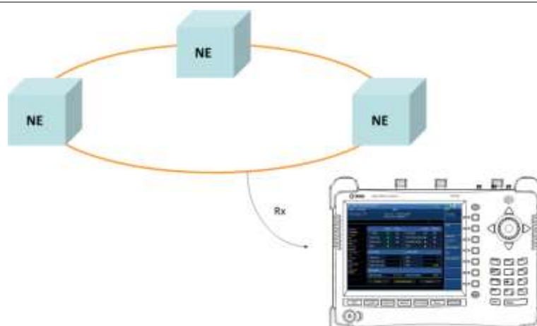
Figure 279 In-service connection
