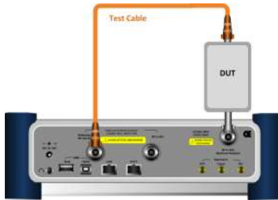
Figure 256 Connection for 2-port scalar measurement
