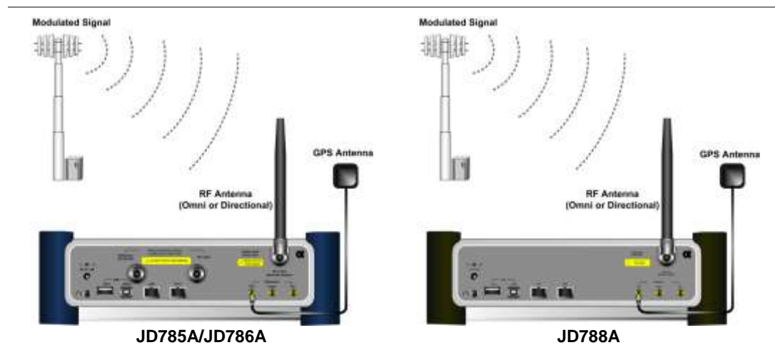
Figure 120 OTA connection
