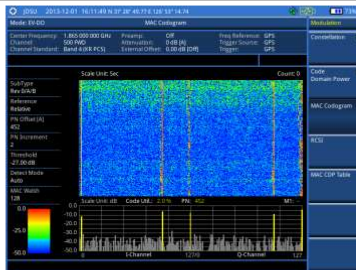
Figure 193 MAC Codogram in full view with EV-DO signal analyzer
