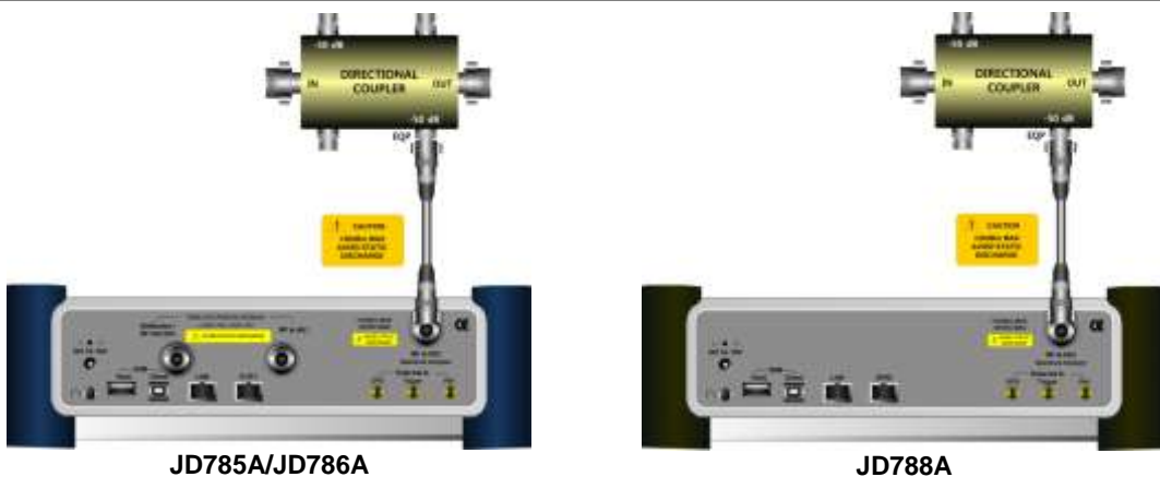
Figure 81 Indirect connection
