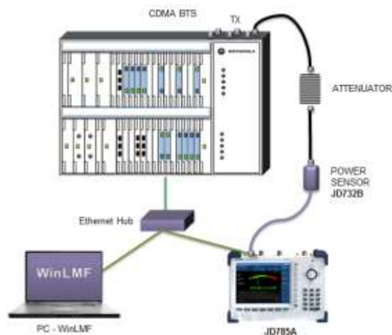
Figure 307 Using external power sensor
