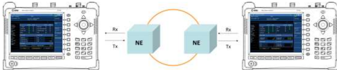
Figure 270 Loop-back connection
