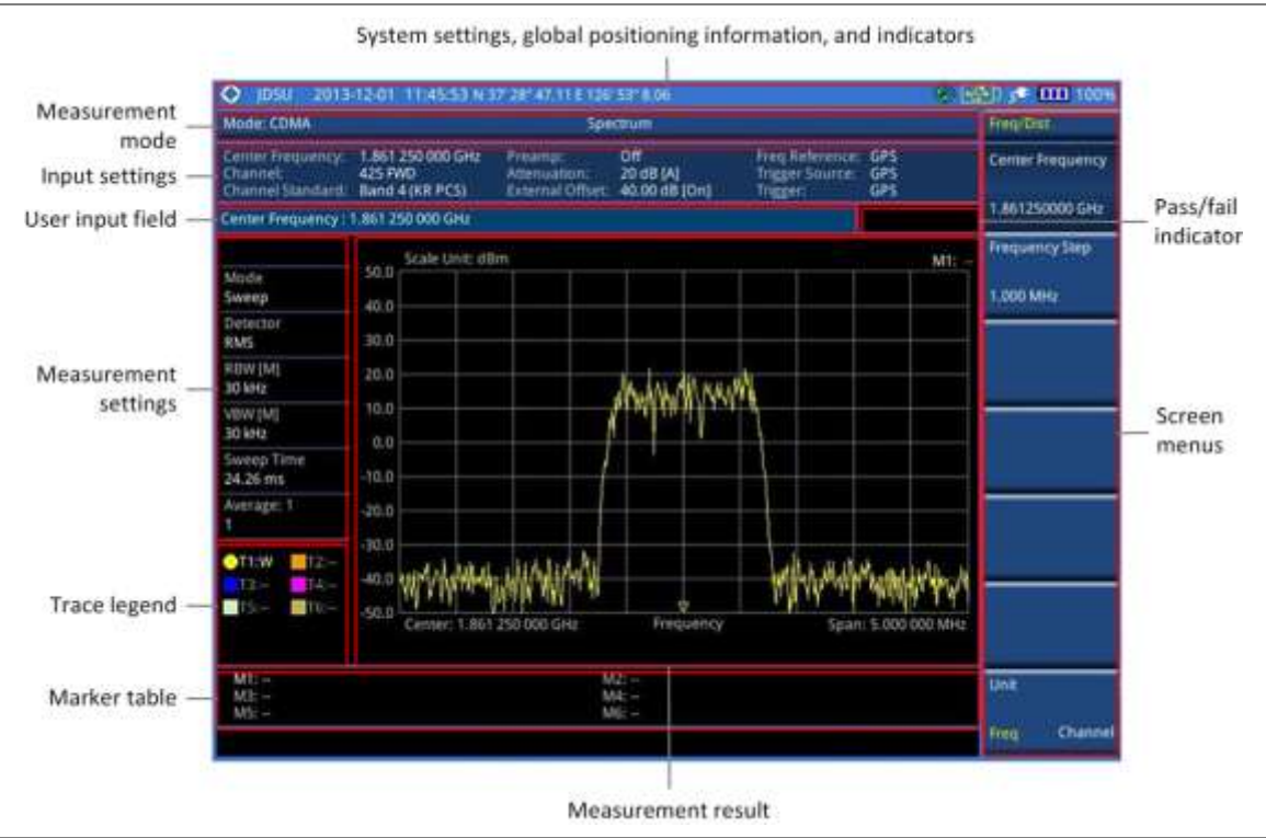
Figure 154 CDMA signal analyzer measurement screen
