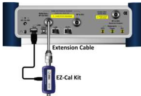
Figure 249 1-port calibration connection with electronic EZ-Cal kit
