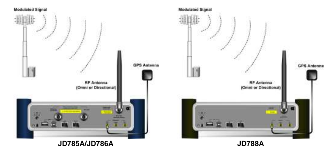
Figure 157 OTA connection
