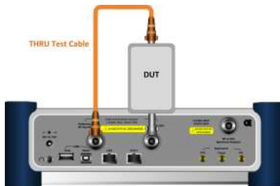
Figure 255 Connection for 2-port vector measurement
