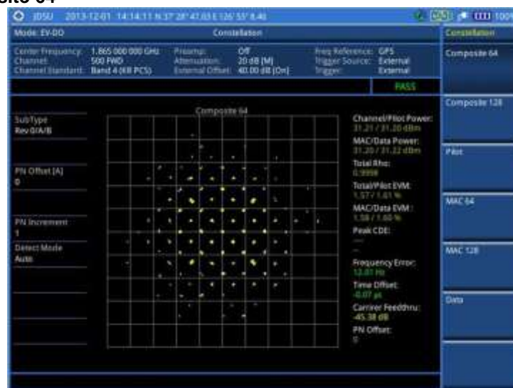
Figure 191 Constellation measurement with EV-DO signal analyzer
