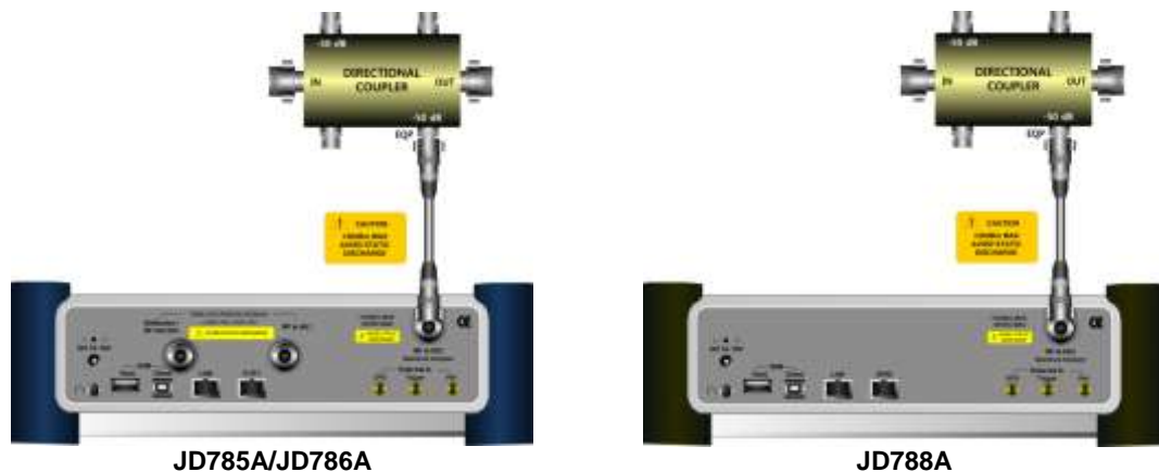
Figure 229 Indirect connection
