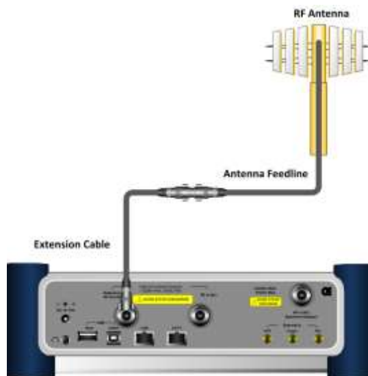
Figure 253 Connection for reflection measurement
