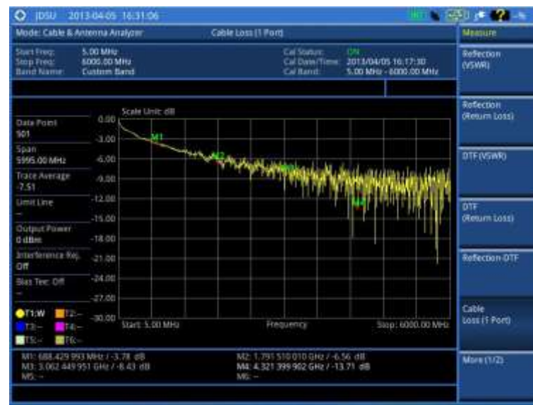
Figure 264 Cable loss (1 port) measurement with zoom
