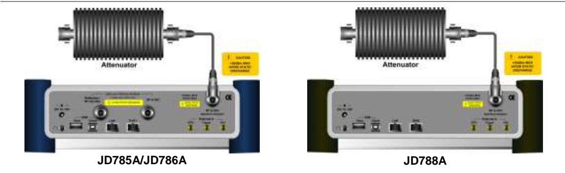
Figure 155 Direct connection
