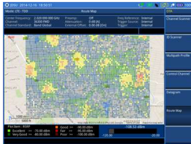
Figure 152 Raster image overlaid on the route map in LTE-TDD OTA signal analyzer
