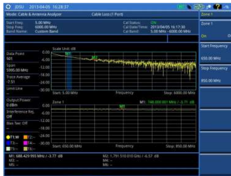
Figure 262 Cable loss (1 port) measurement with the zone enabled
