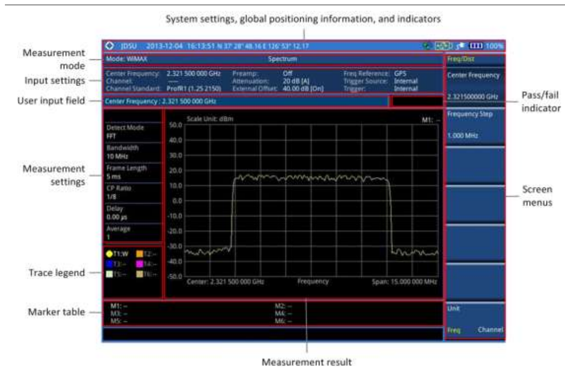
Figure 227 Mobile WiMAX signal analyzer measurement screen
