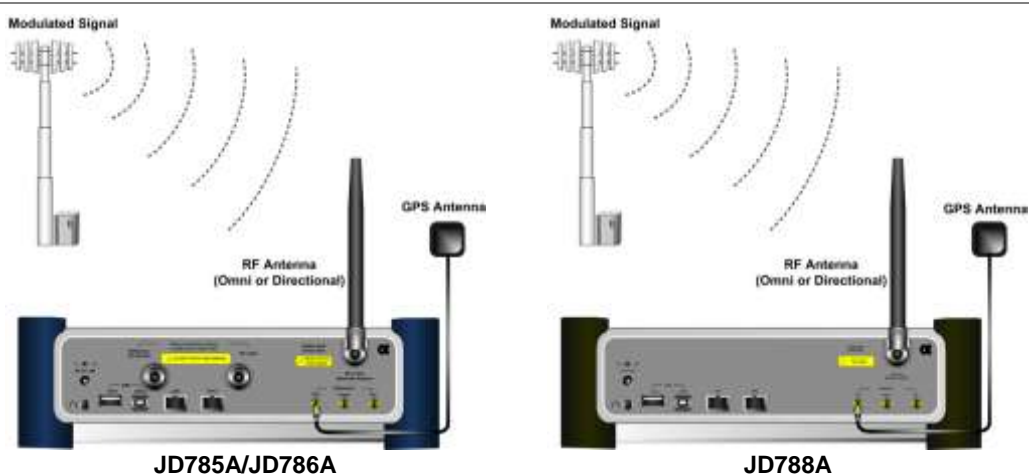
Figure 180 OTA connection
