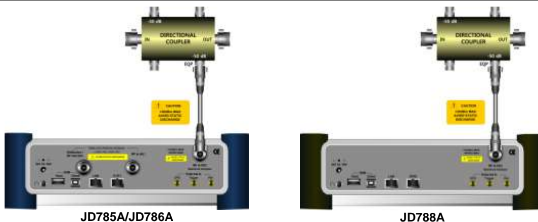
Figure 293 Indirect connection
