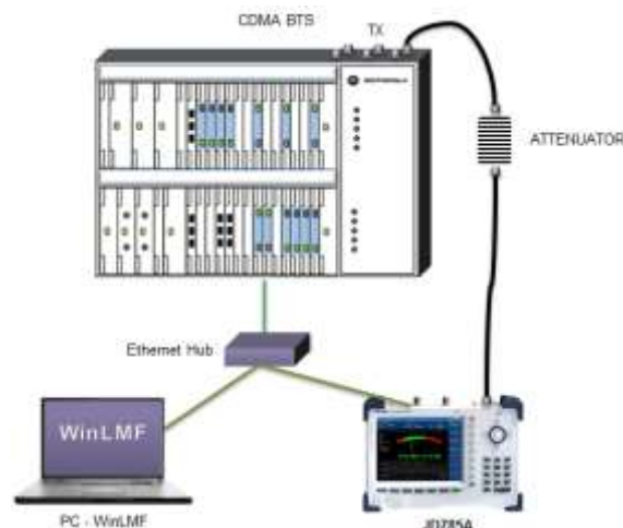
Figure 306 Using internal power sensor
