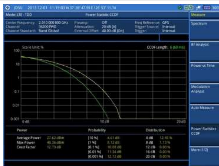
Figure 143 CCDF measurement with LTE - TDD signal analyzer
