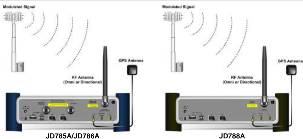
Figure 230 OTA connection
