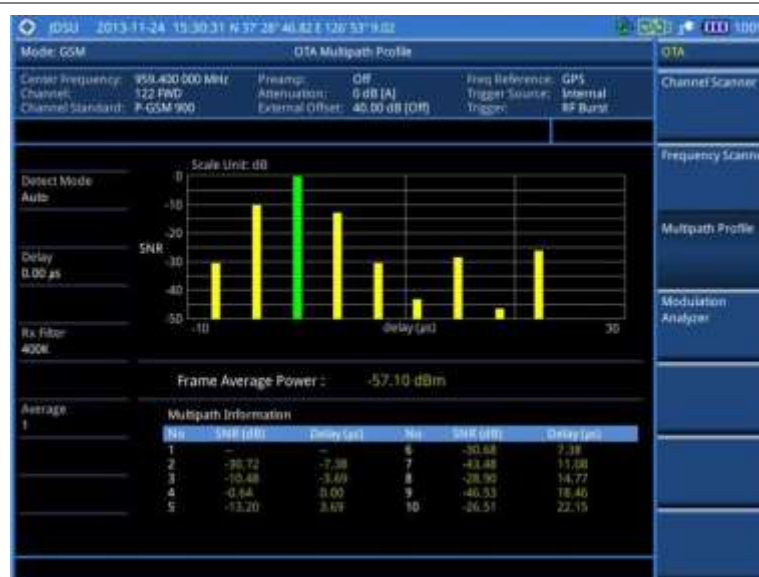
Figure 52 Multipath profile measurement with GSM OTA signal analyzer
