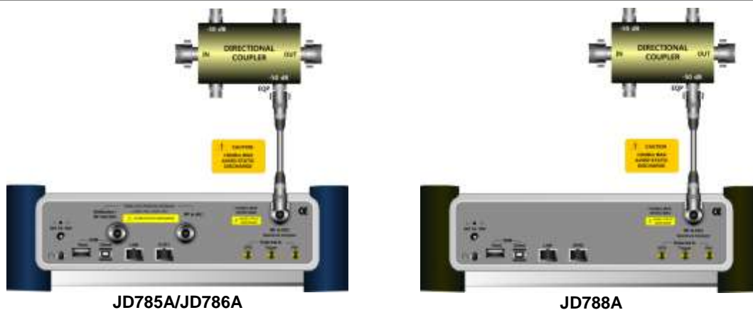
Figure 156 Indirect connection
