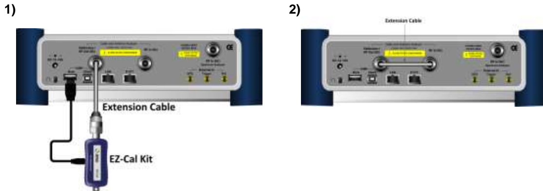
Figure 251 2-port calibration connection with EZ-Cal in vector measurements
