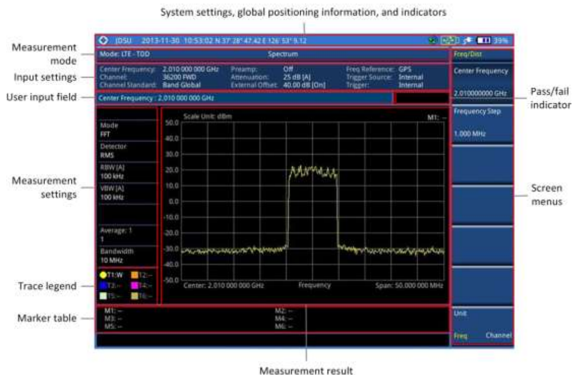
Figure 117 LTE - TDD signal analyzer measurement screen
