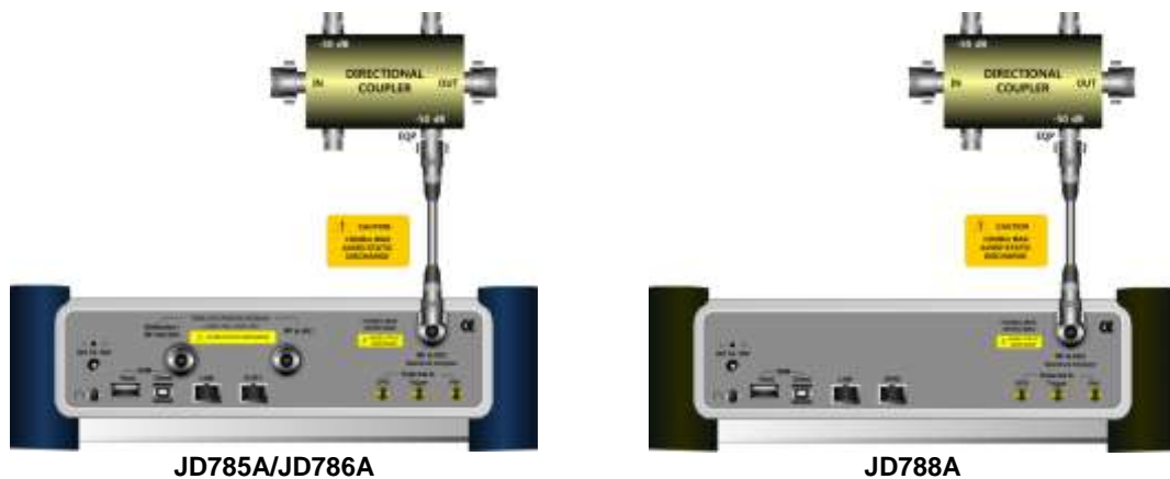
Figure 10 Indirect connection
