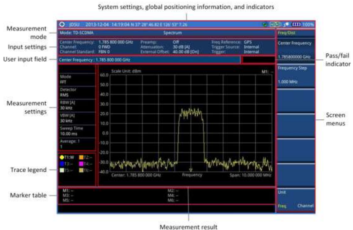
Figure 202 TD-SCDMA signal analyzer measurement screen
