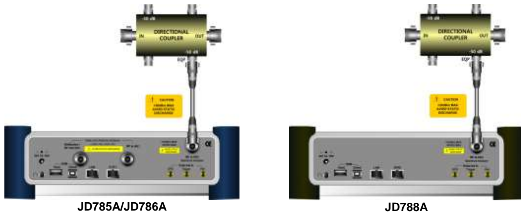
Figure 204 Indirect connection
